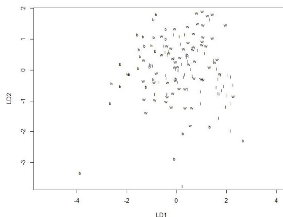
Fig. 1: Linear discriminant representation of the three plumage colour variants in Nigerian local turkeys. w = white plumage, l = lavender plumage, b = black plumage.
